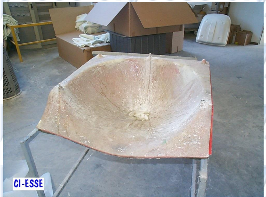
Cover chair production site RTM light By Ci-ESSE aluminium molds
